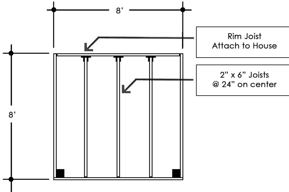
Deck Framing Layout
