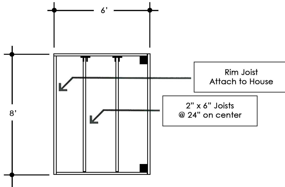
Deck Framing Layout
