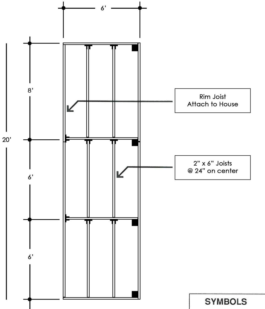
Deck Framing Layout
