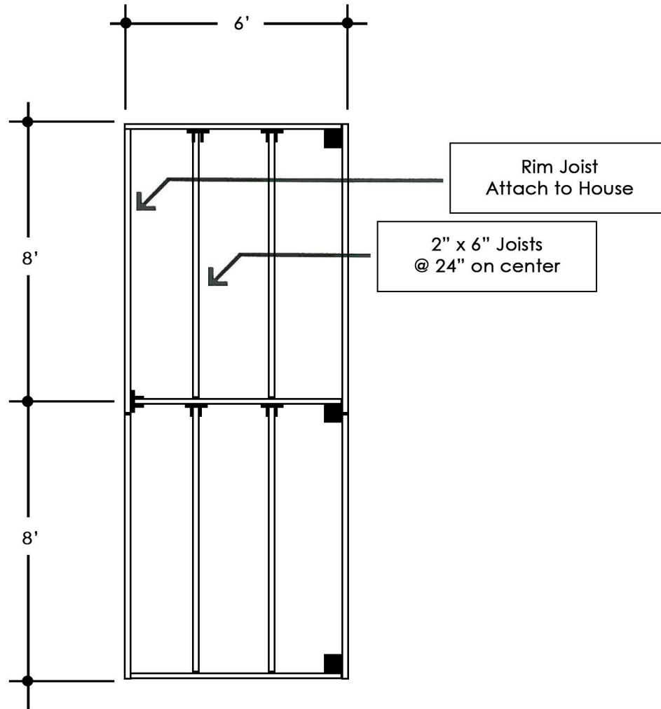
Deck Framing Layout
