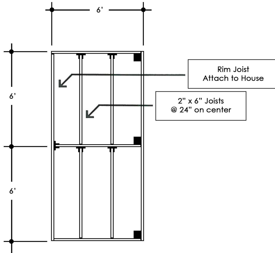
Deck Framing Layout
