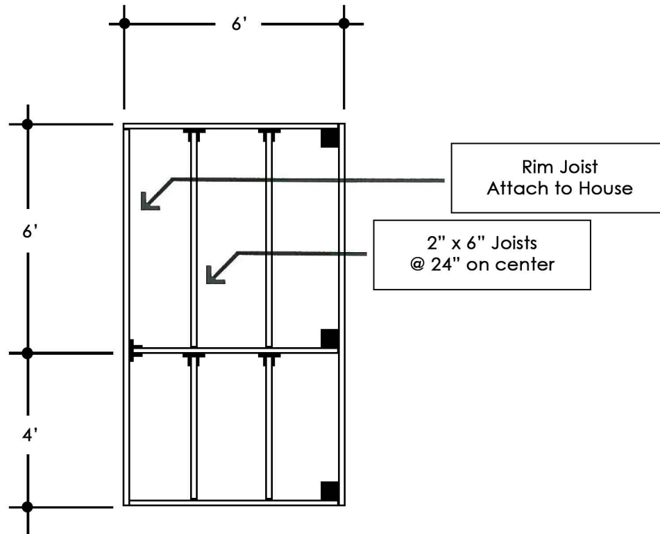
Deck Framing Layout
