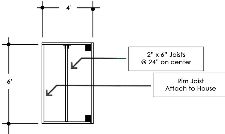
Deck Framing Layout
