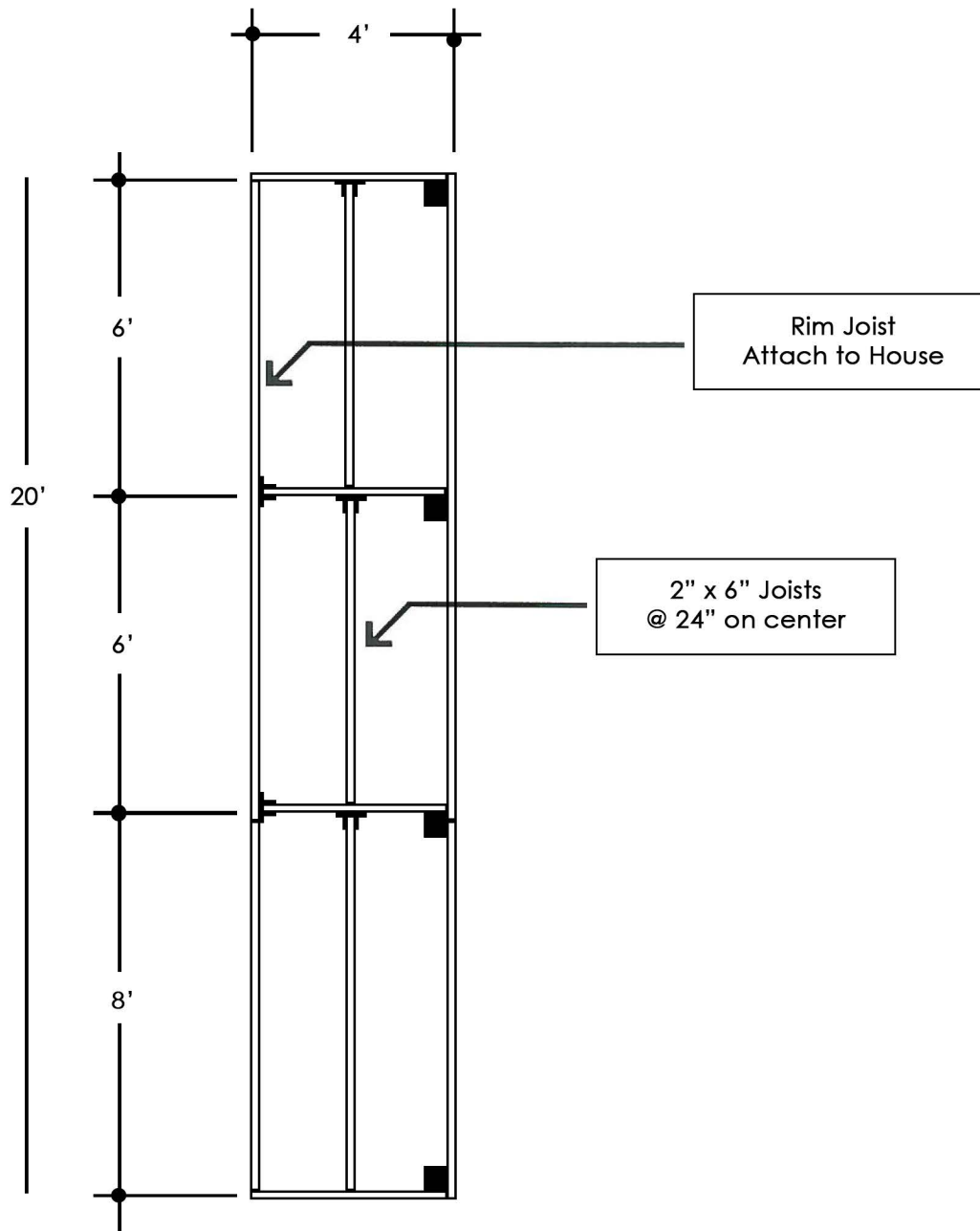
Deck Framing Layout
