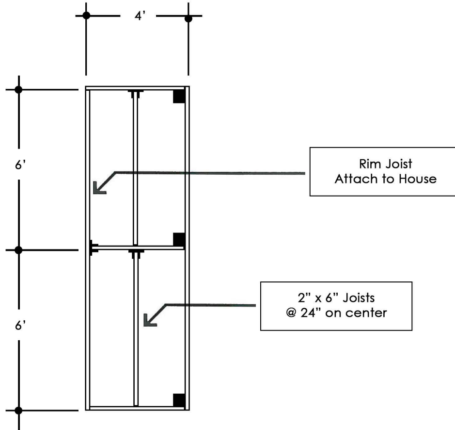
Deck Framing Layout
