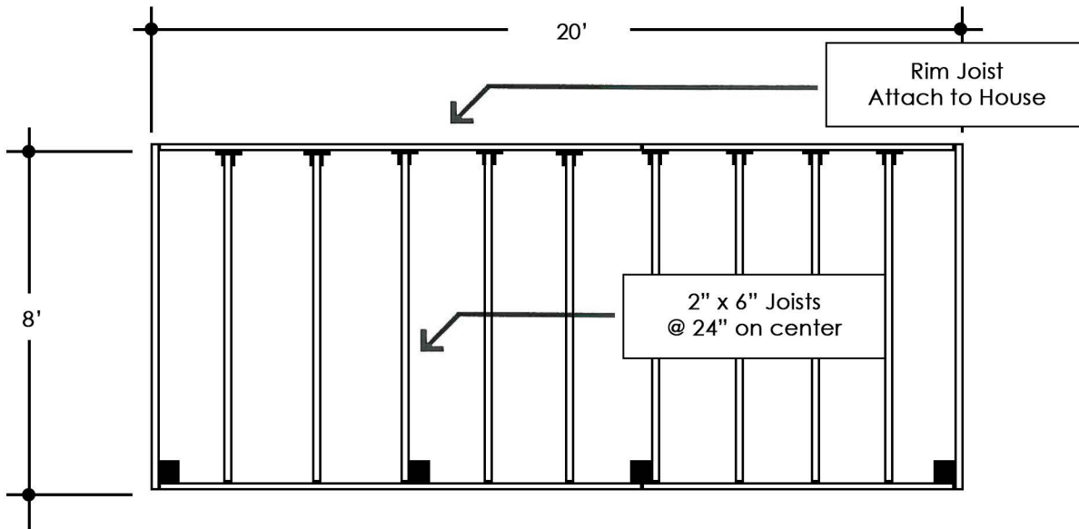
Deck Framing Layout
