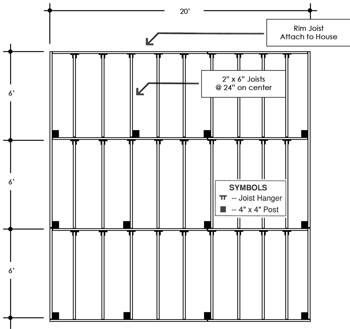
Deck Framing Layout
