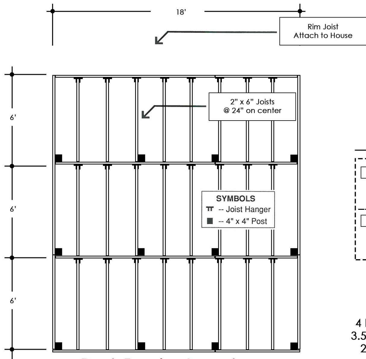
Deck Framing Layout
