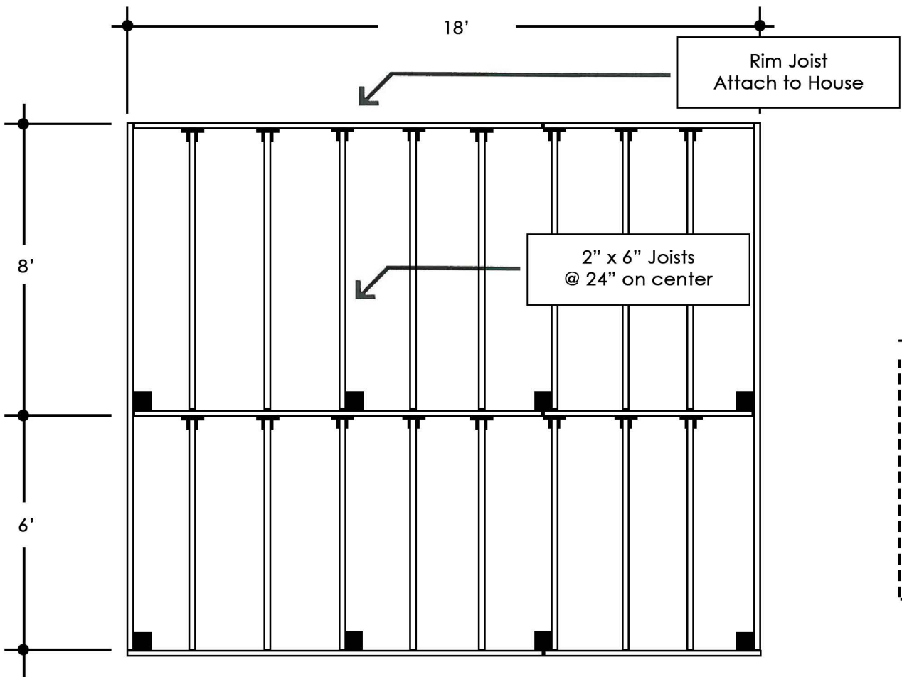
Deck Framing Layout
