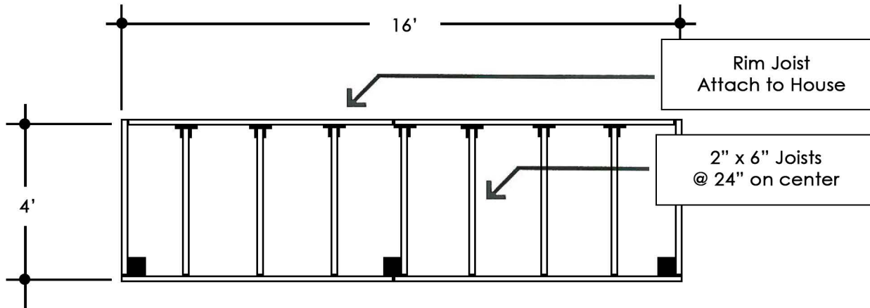
Deck Framing Layout
