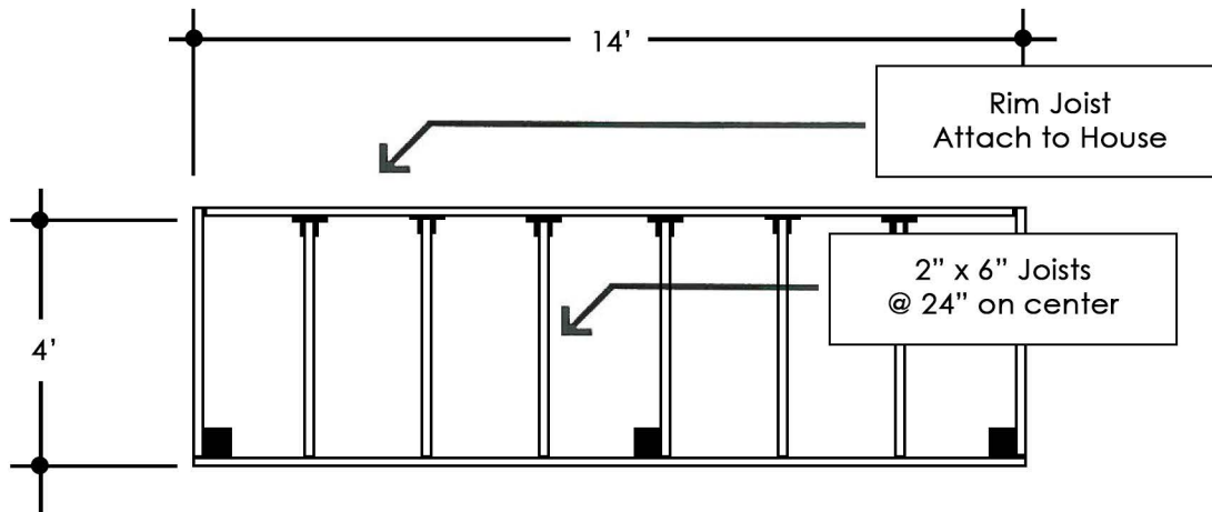
Deck Framing Layout
