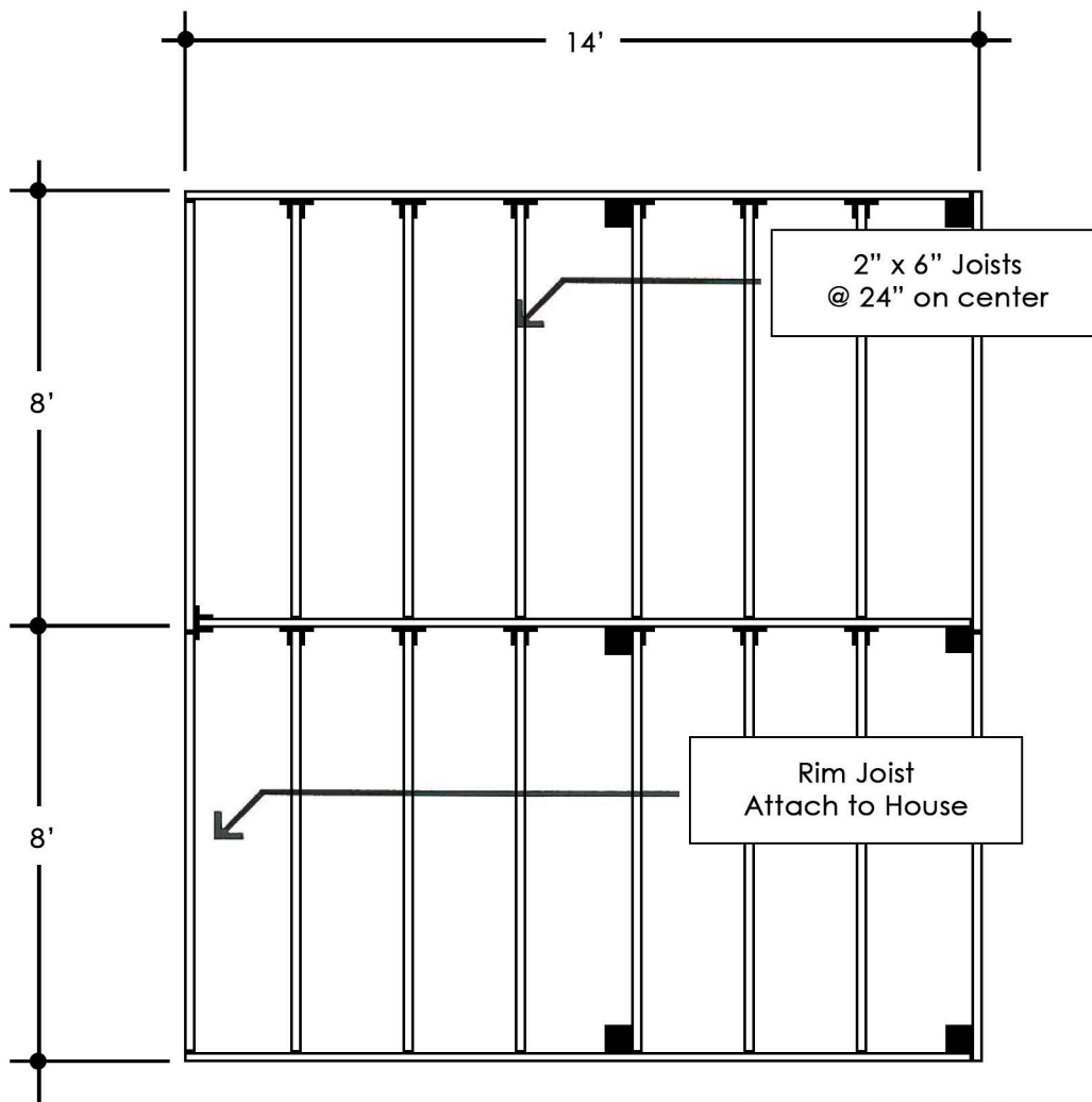
Deck Framing Layout
