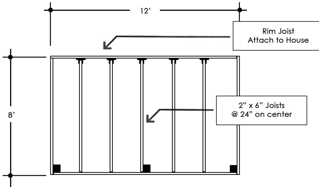
Deck Framing Layout
