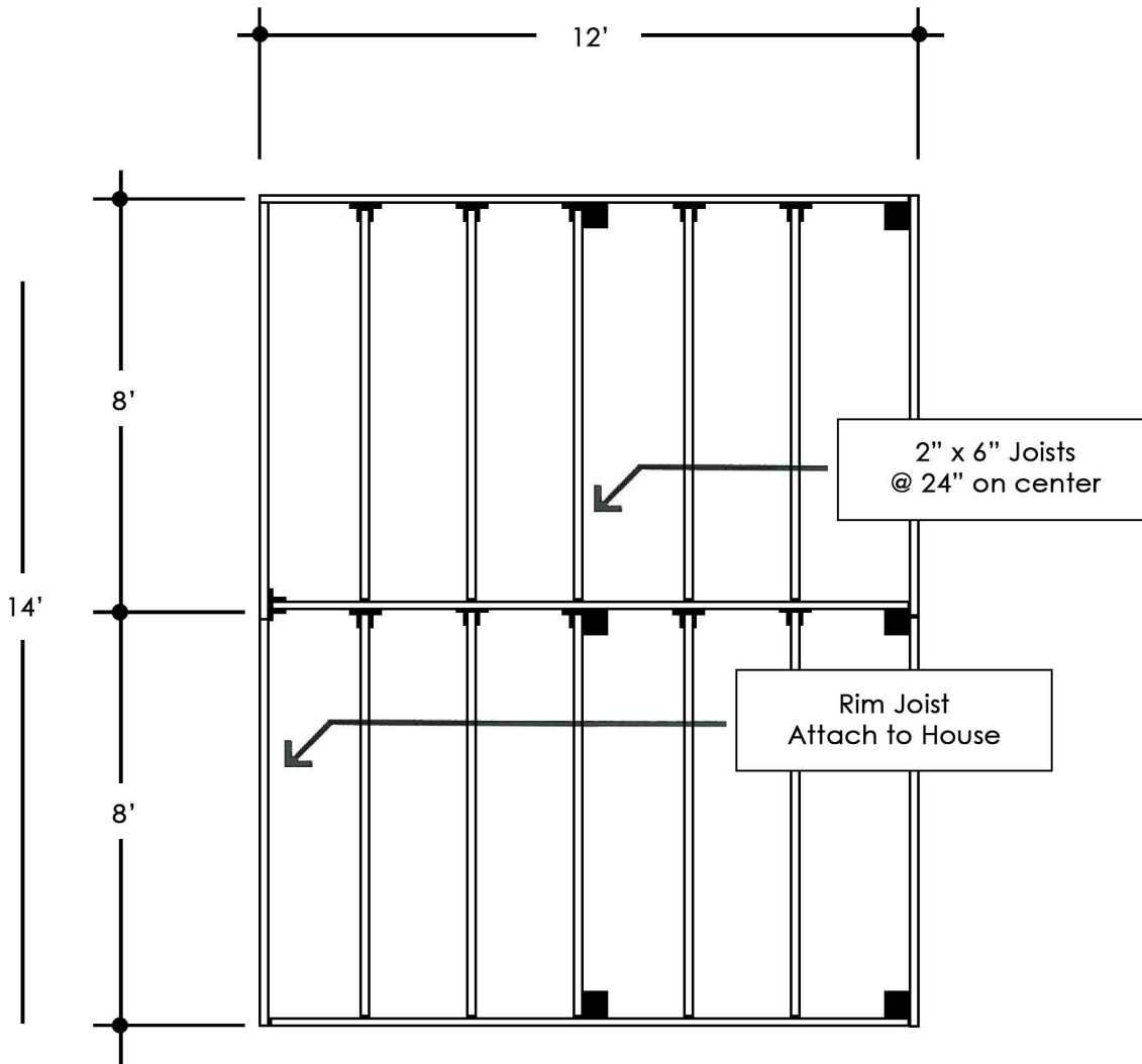
Deck Framing Layout
