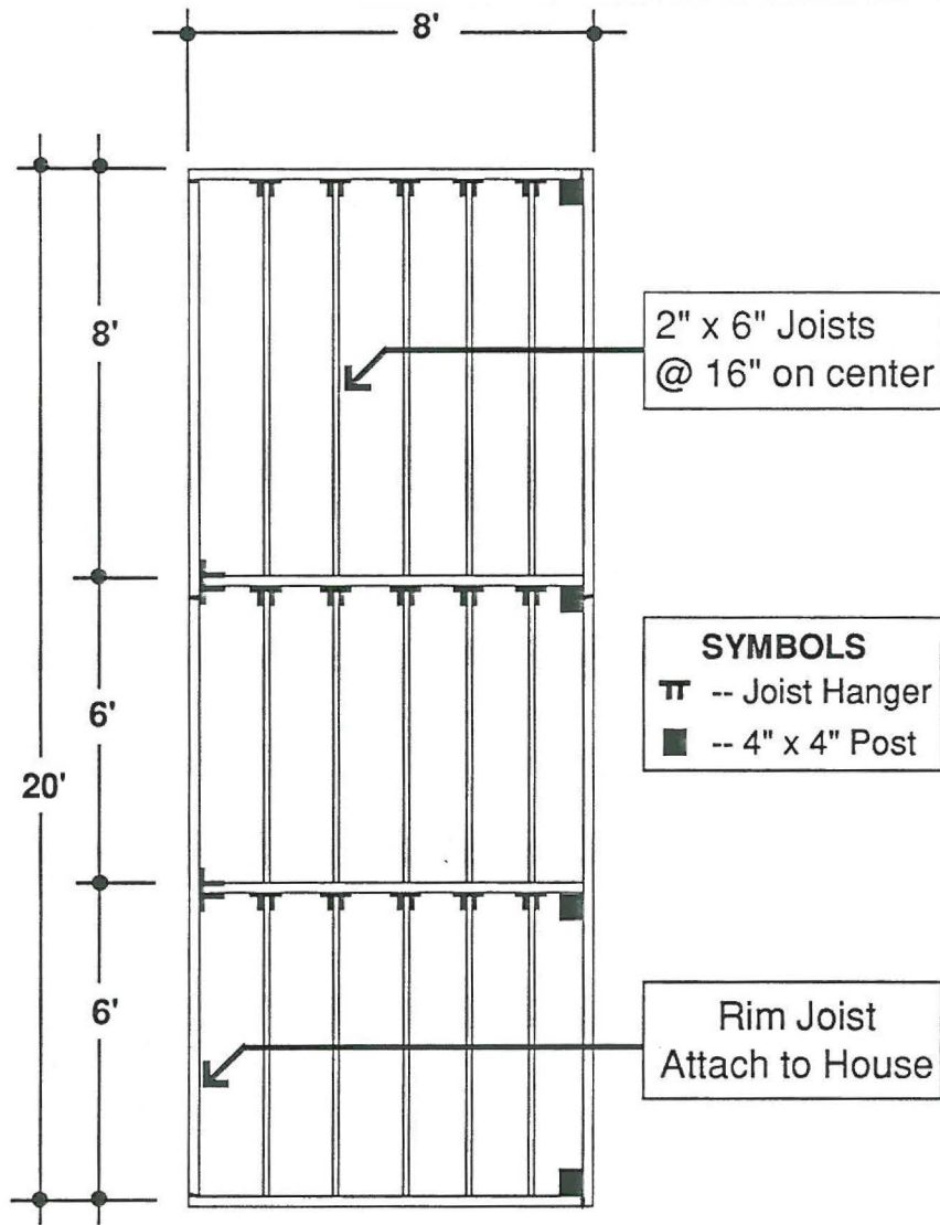
Deck Framing Layout
