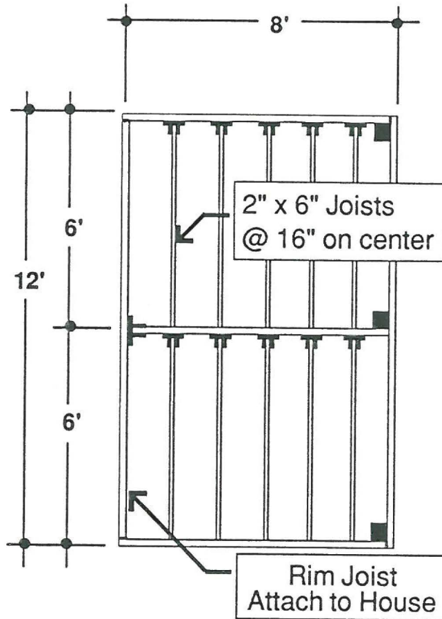
Deck Framing Layout
