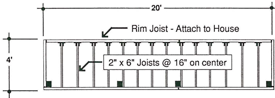
Deck Framing Layout
