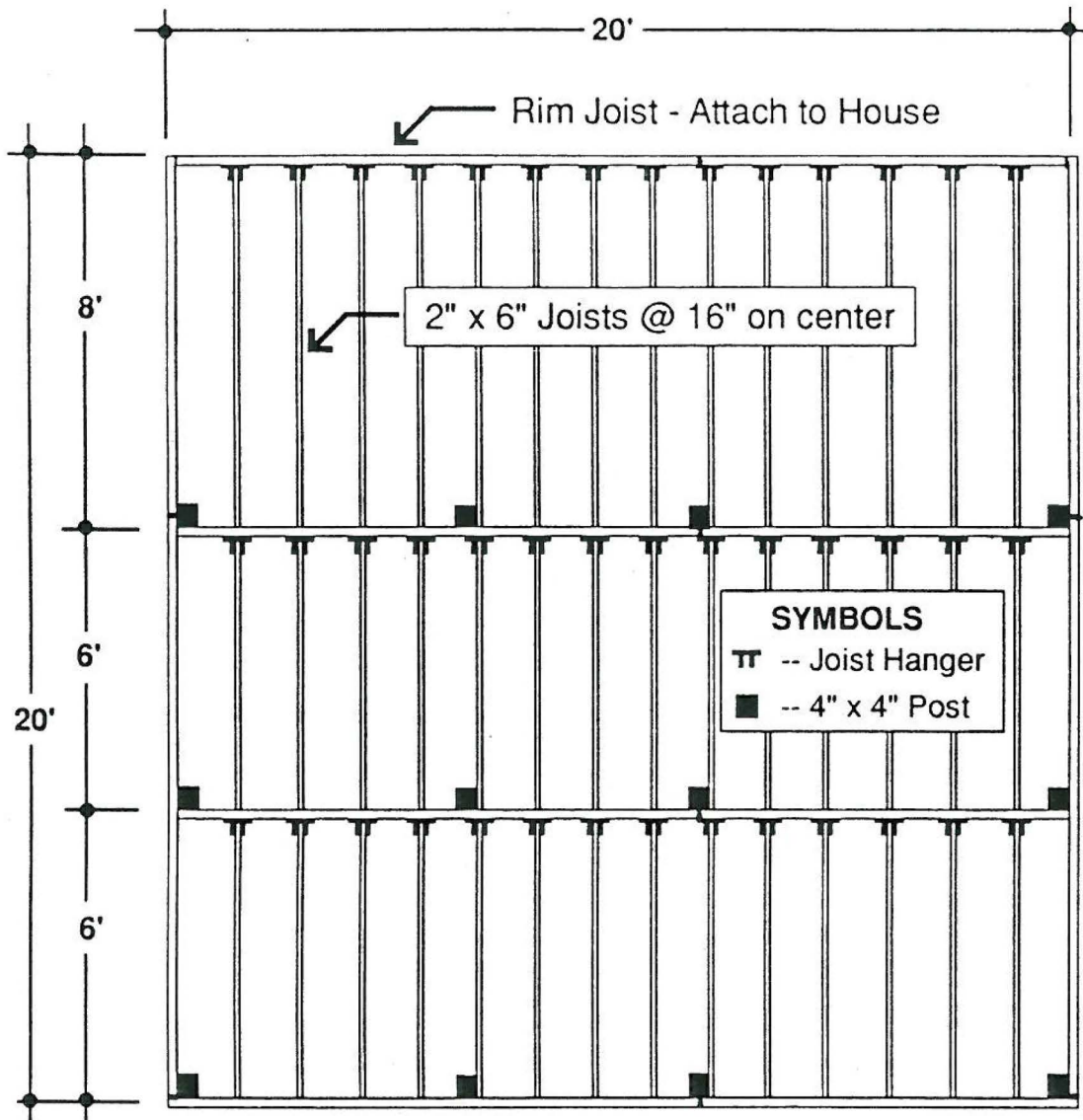
Deck Framing Layout
