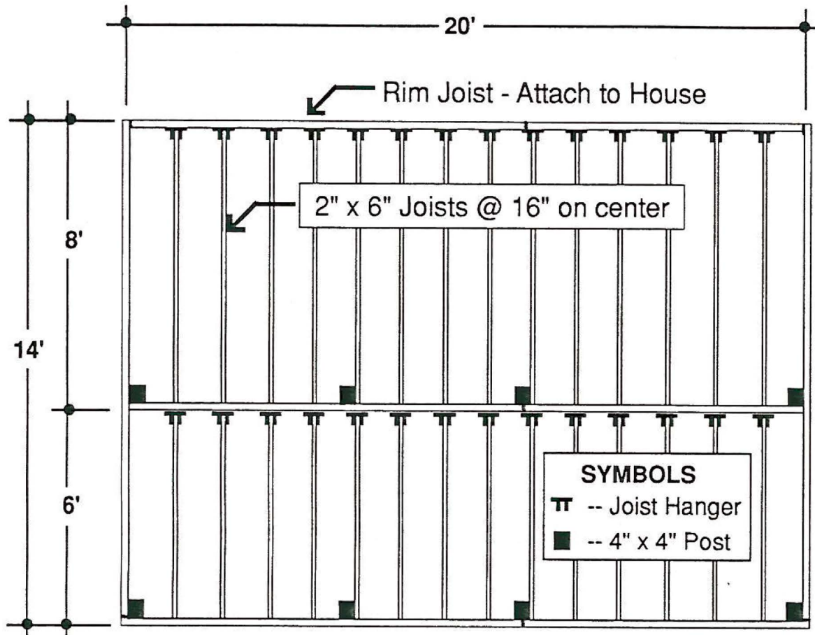
Deck Framing Layout
