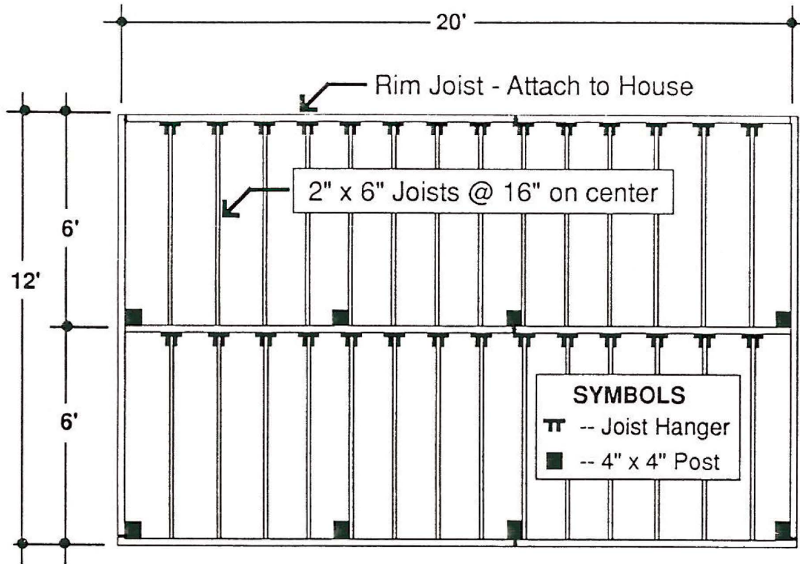
Deck Framing Layout
