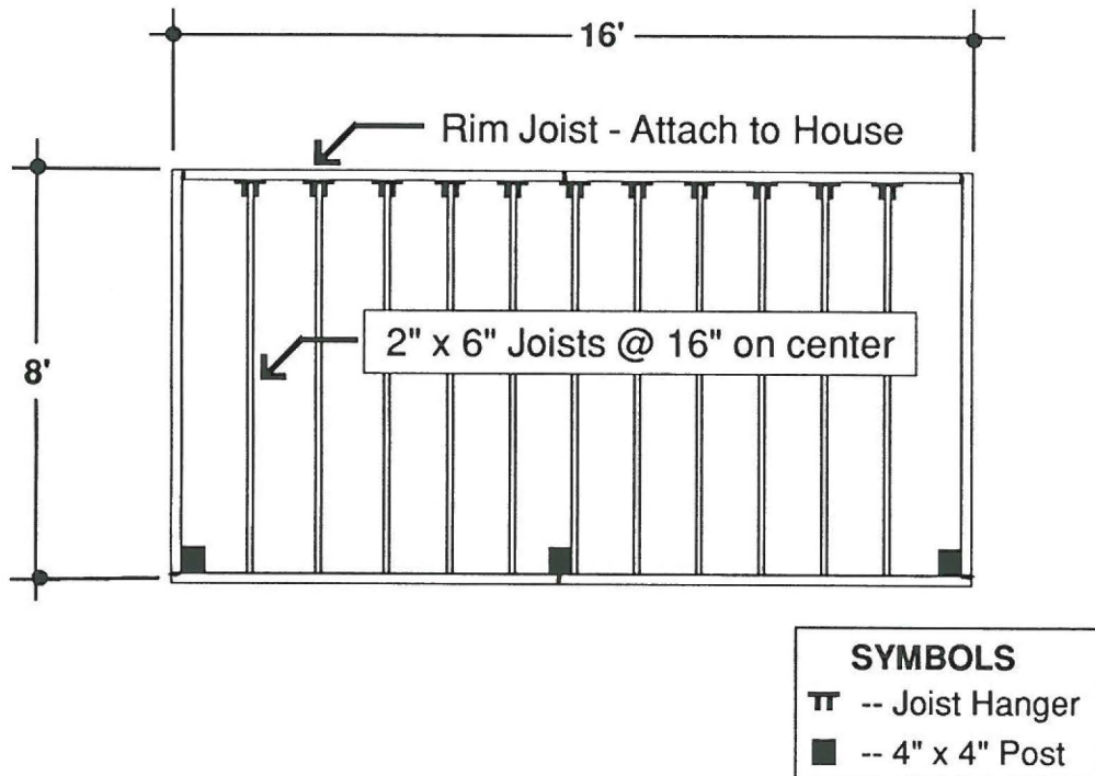
Deck Framing Layout
