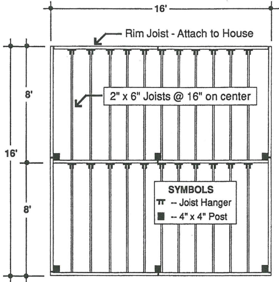
Deck Framing Layout
