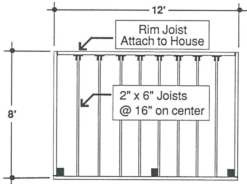
Deck Framing Layout
