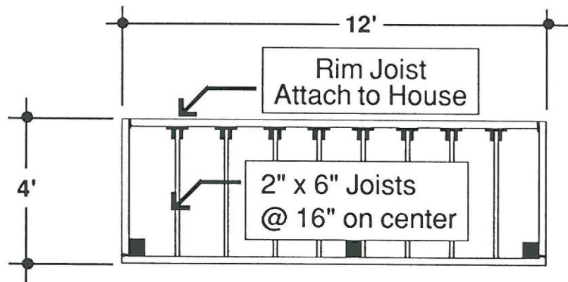
Deck Framing Layout
