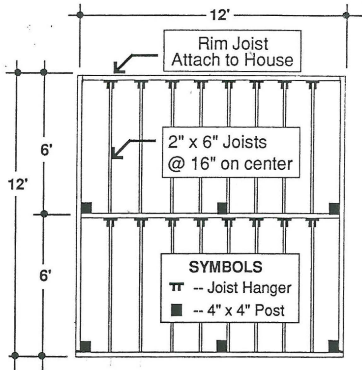
Deck Framing Layout
