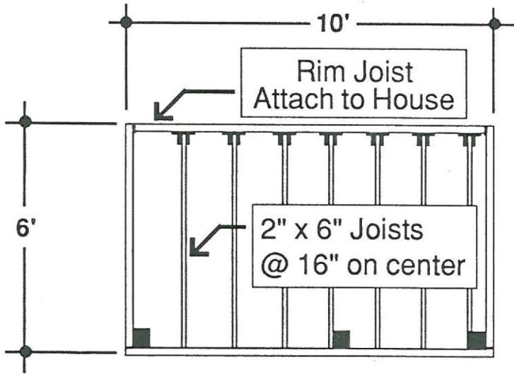
Deck Framing Layout
