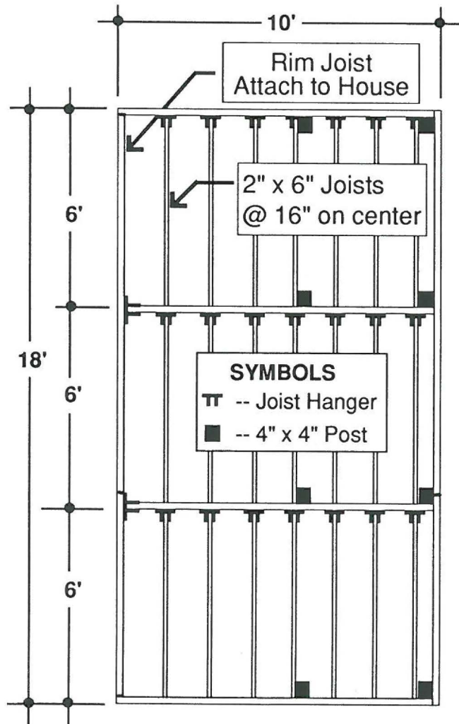
Deck Framing Layout
