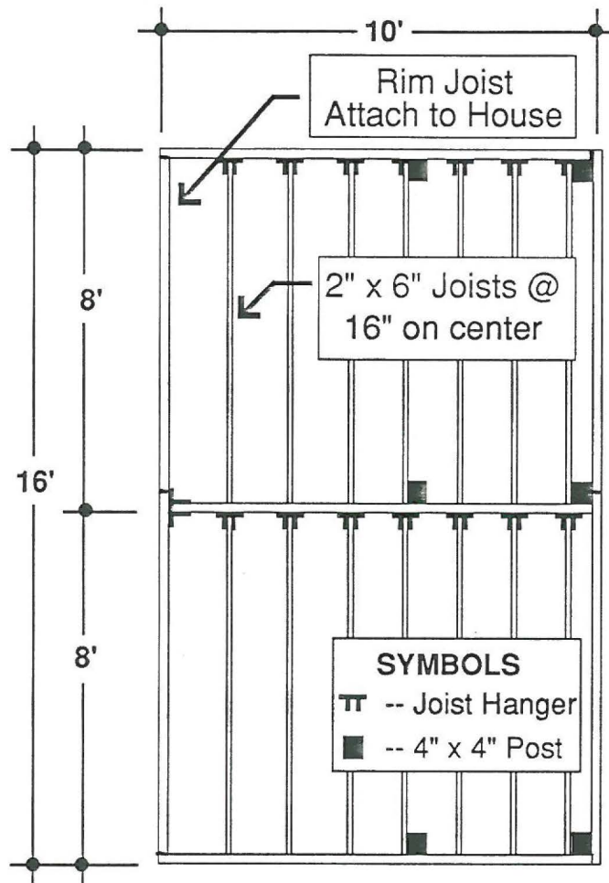
Deck Framing Layout
